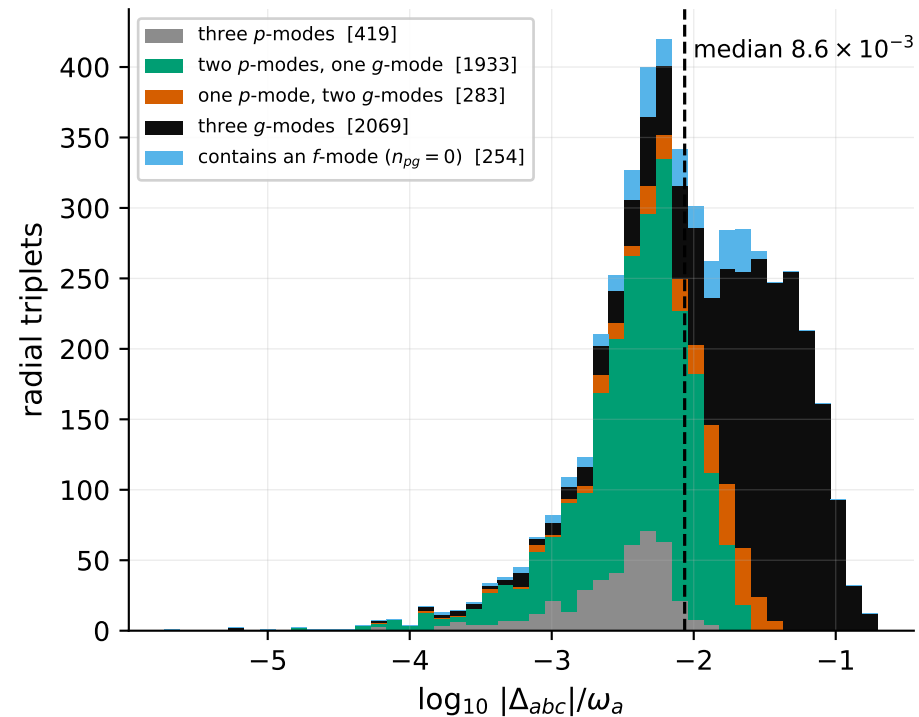
(a) 4958 radial triplets by p/g make-up
